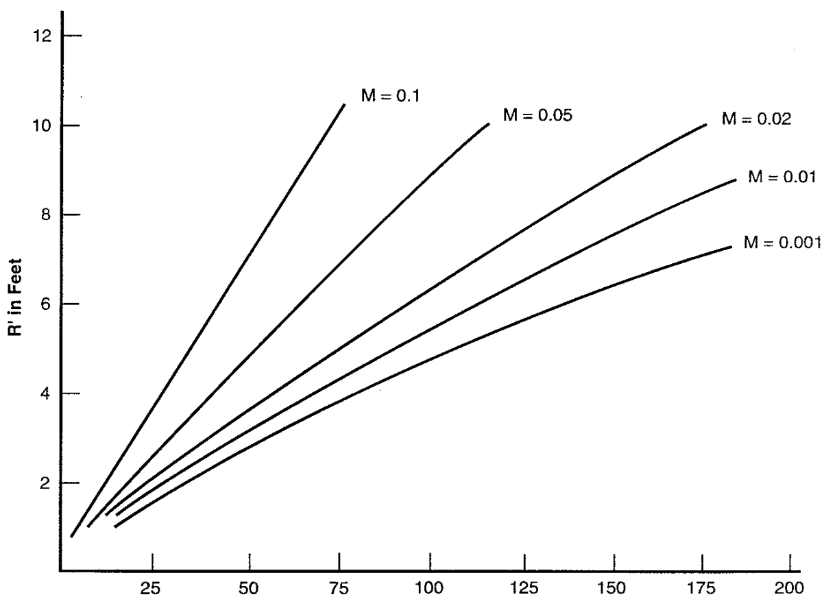
Figure D-17. Curves for Computation of Runup Inland of Low Bluffs
