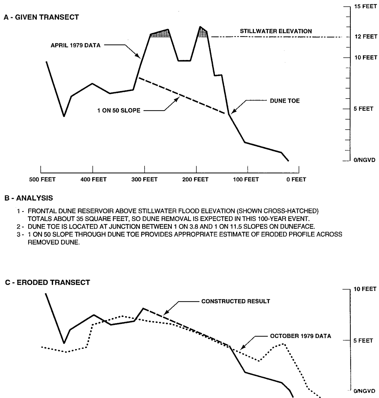
Figure D-6. Quantitative Example of Dune Removal Treatment for Alabama Profile Eroded by 1979 Hurricane Frederic. Situation Is Profile B-35 in Baldwin County, Alabama
